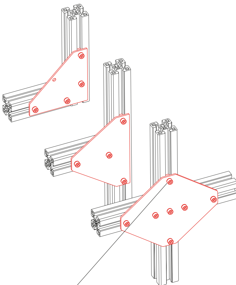
Fixing set
